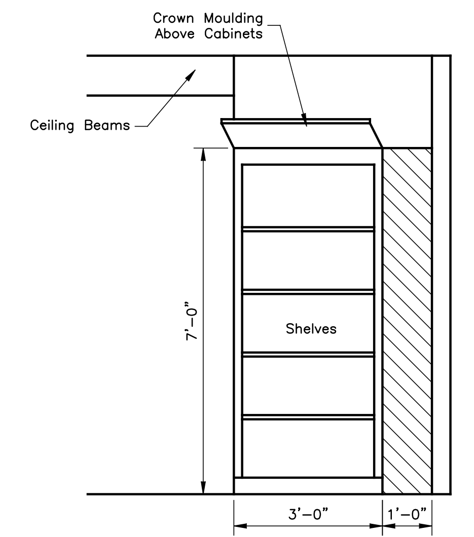
LIVING ROOM BOOK CASE SCALE: 1/2"=1'-0"
