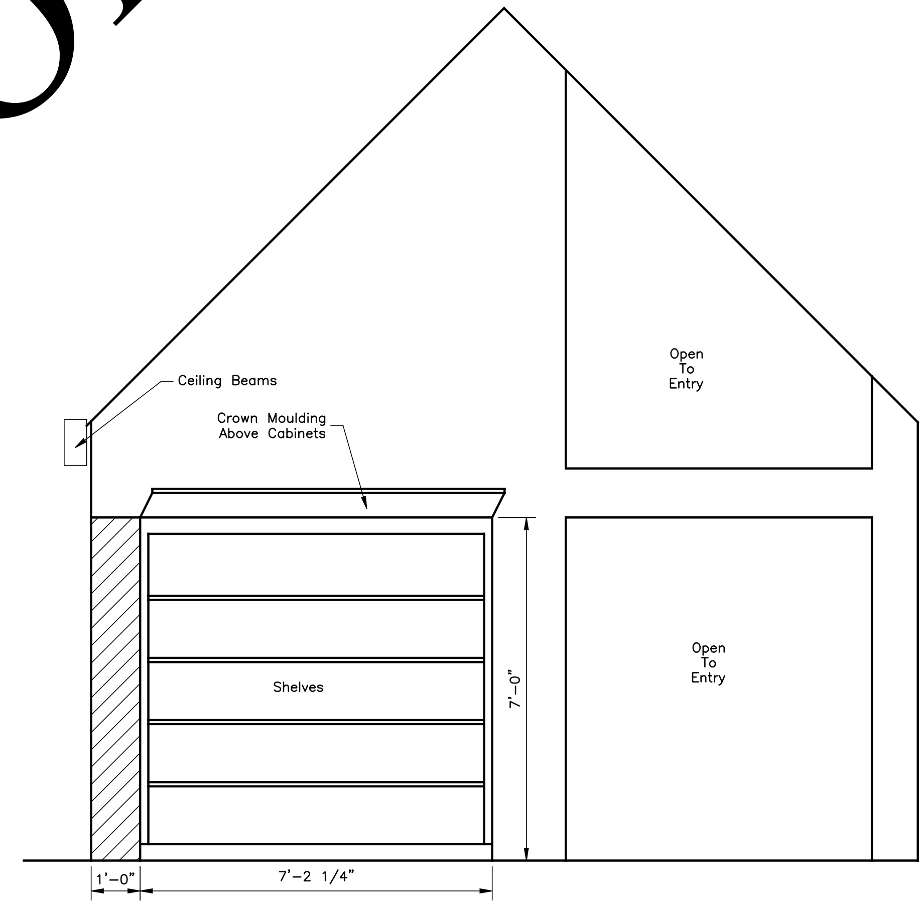
LIVING ROOM BOOK CASE SCALE: 1/2"=1'-0"
