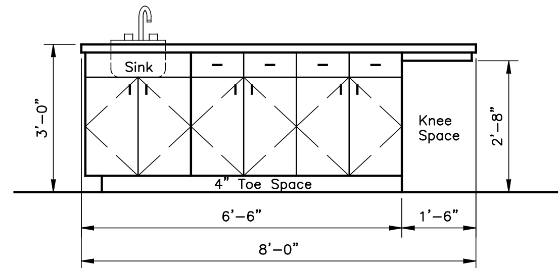
KITCHEN BAR FRONT SCALE: 1/2"=1'-0"
