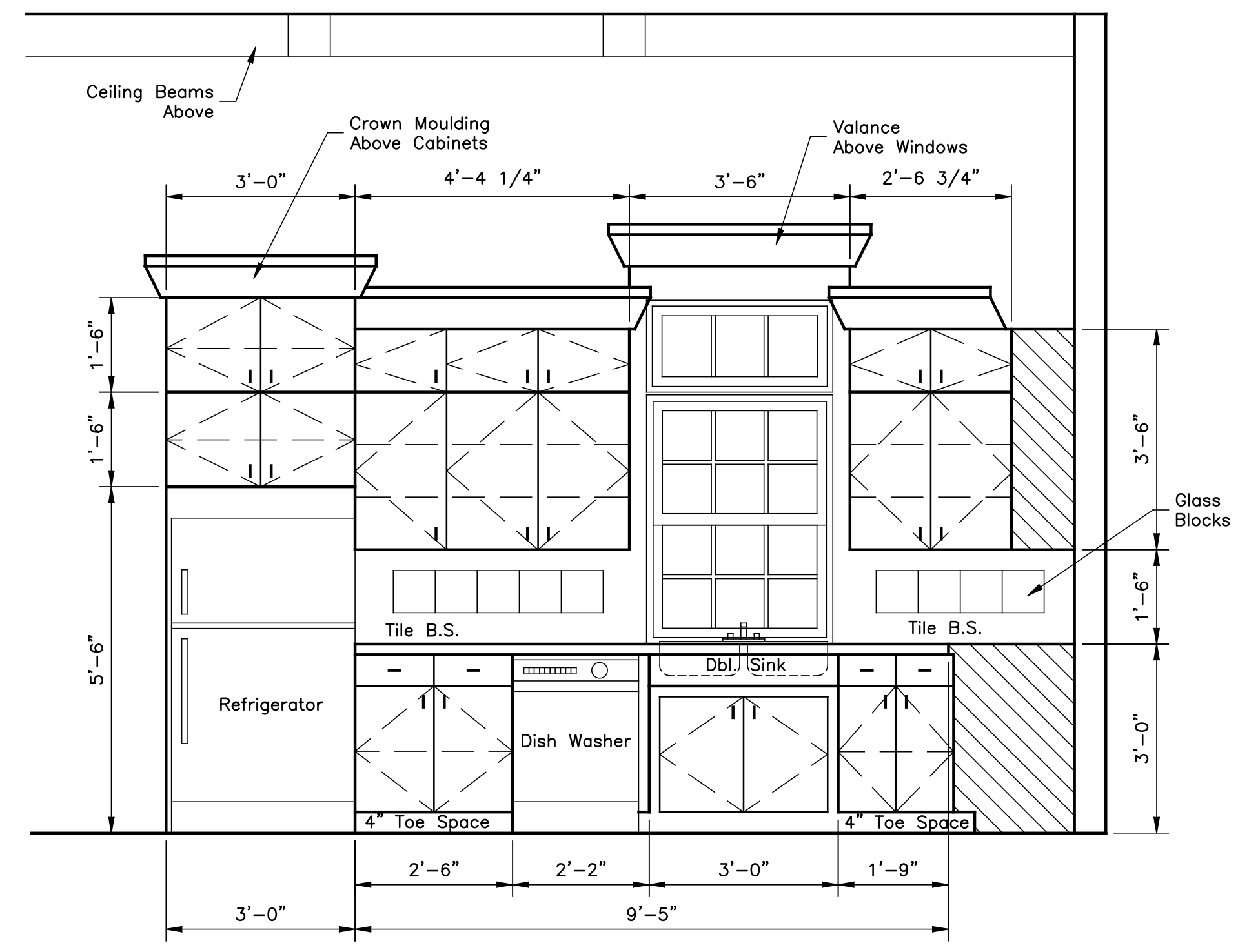
KITCHEN SINK & FRIG SCALE: 1/2"=1'-0"
